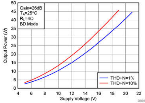
(Load=4Ω, Fsw=480kHz, High Performance Mode)
