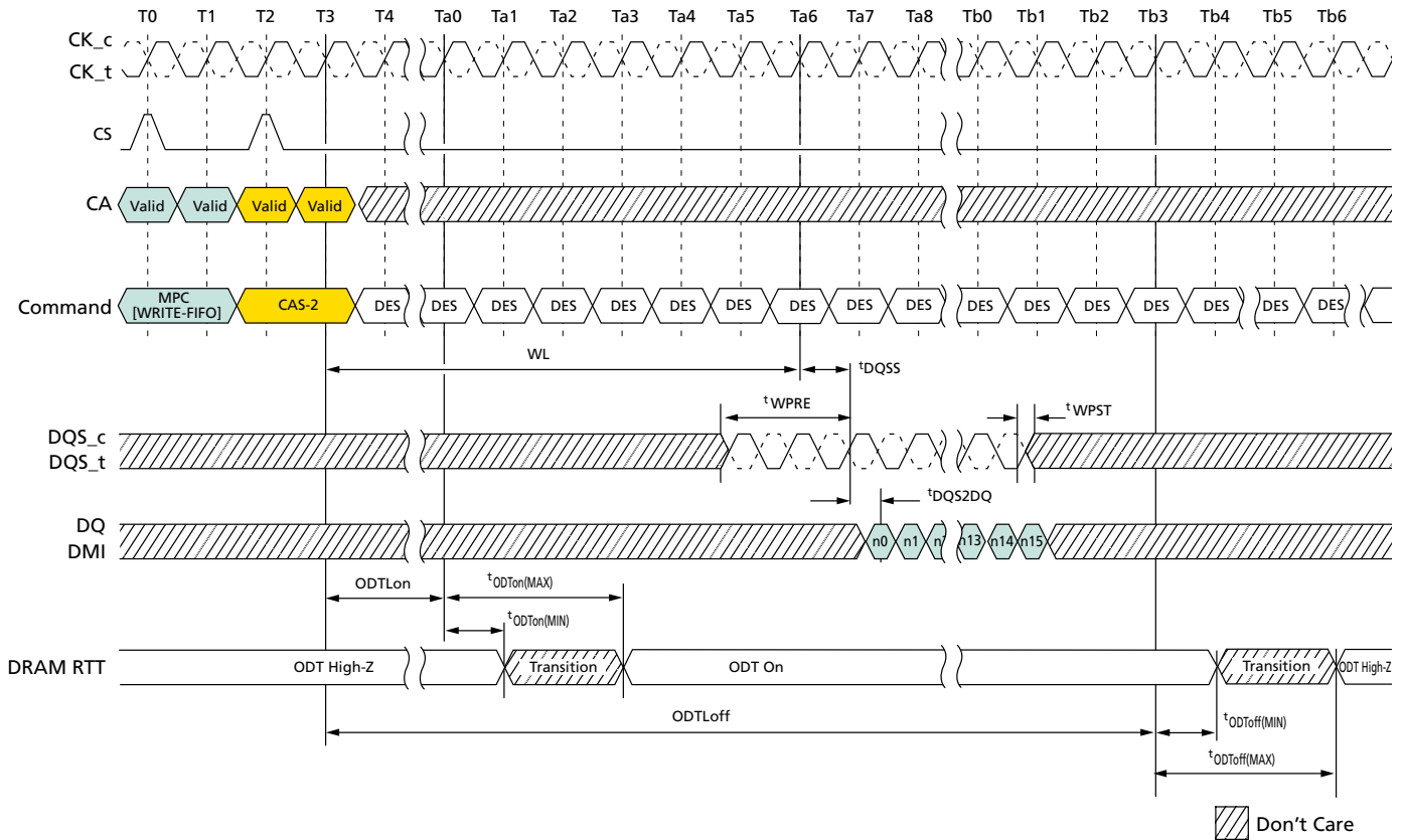
Figure 114: MPC[WRITE-FIFO] with DQ ODT Timing
