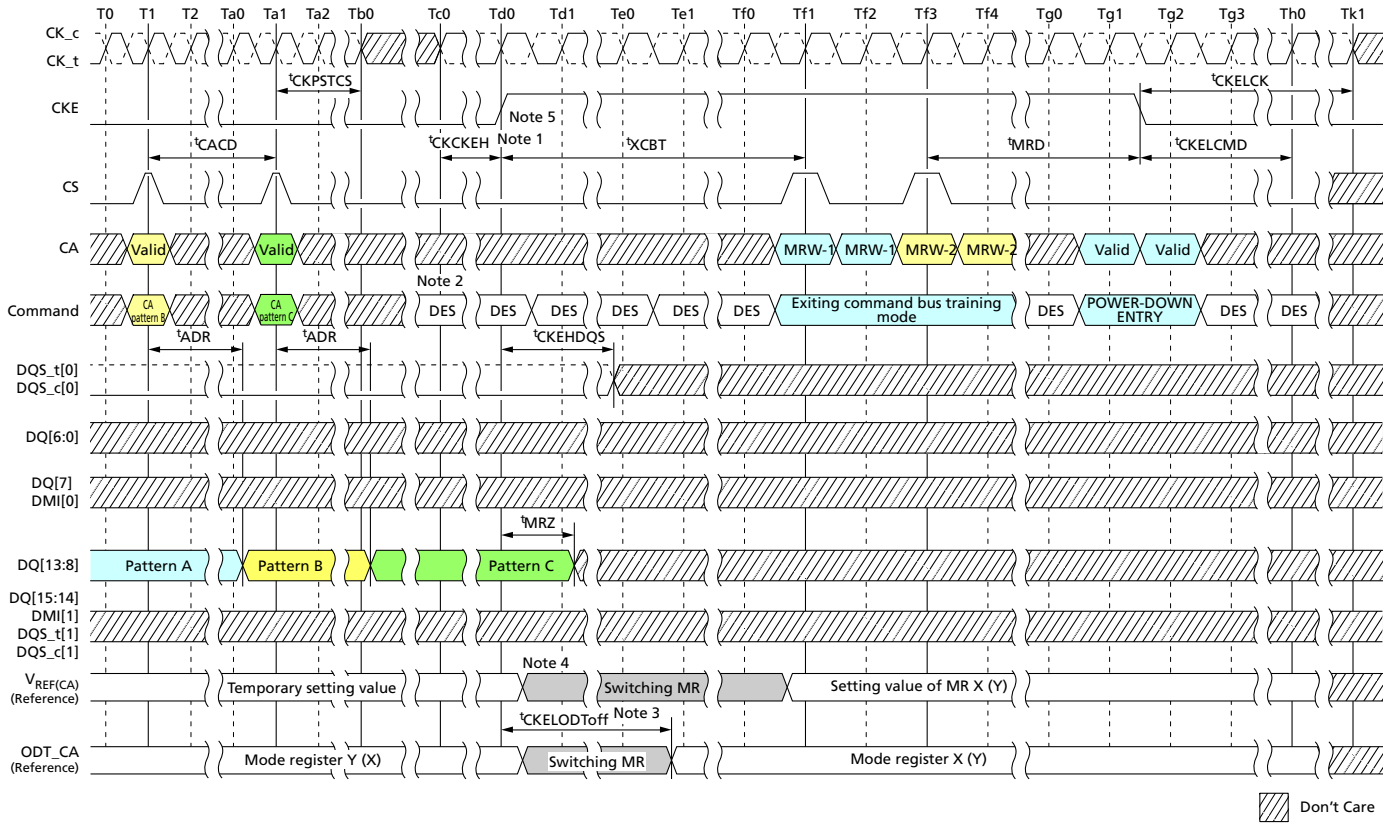
Figure 100: Command Bus Training Mode Exit with Power-Down Entry
