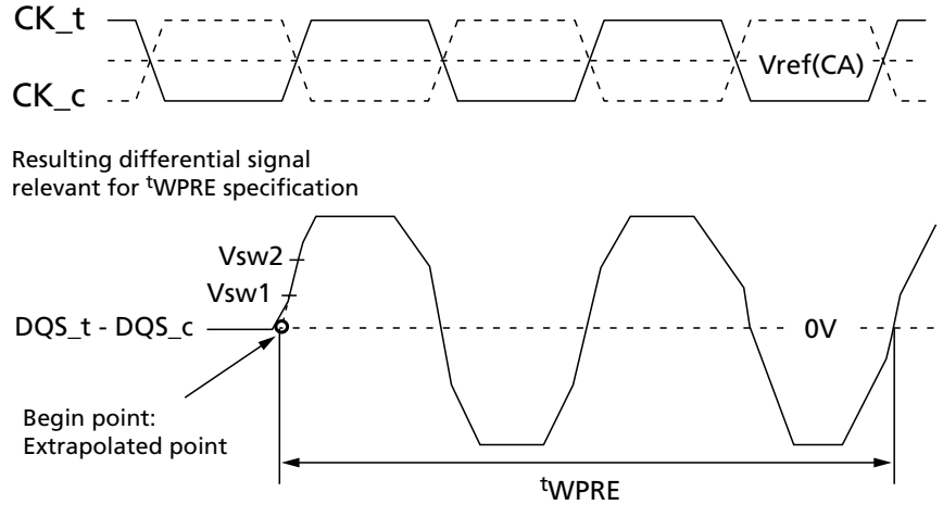
Figure 28: Method for Calculating t_{WPRE} Transitions and Endpoints
