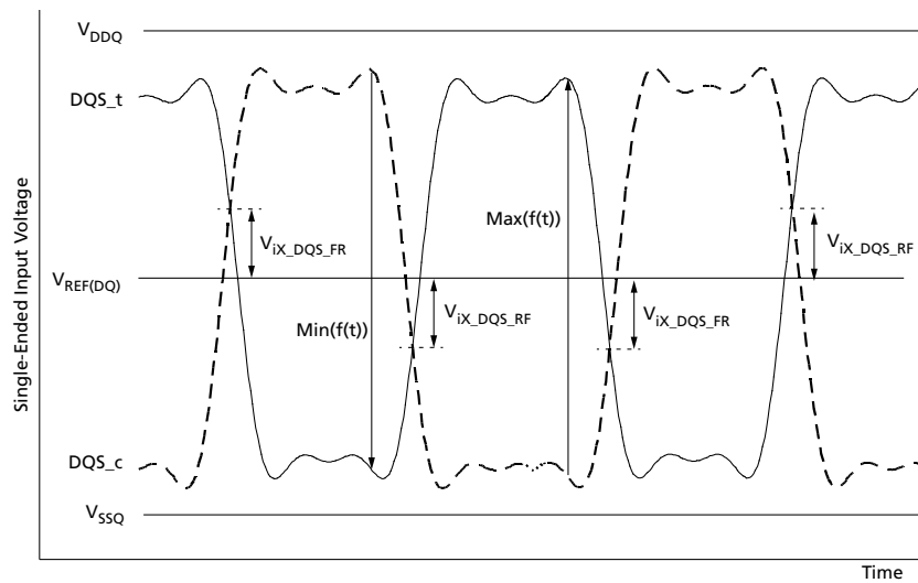
Figure 142: V_{IX} Definition (DQS)
