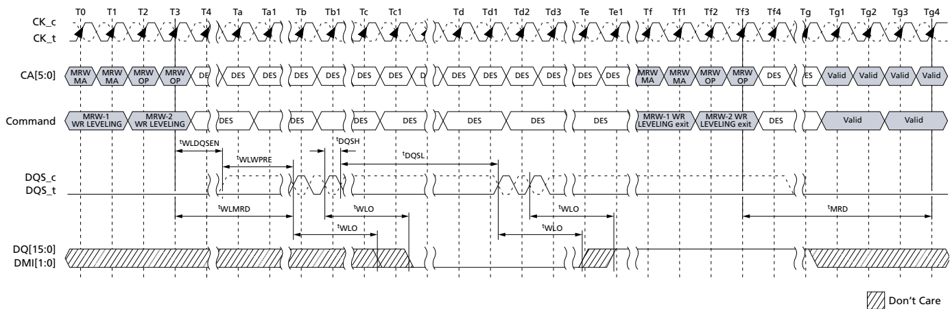
Figure 101: Write Leveling Timing – t_{DQSL}(\text{MAX})
