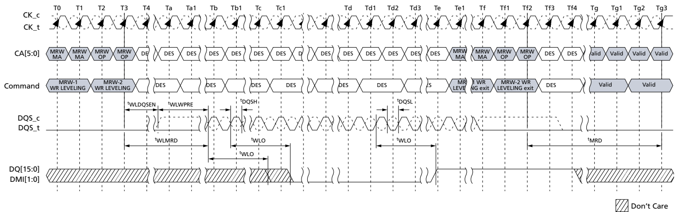
Figure 102: Write Leveling Timing – t_{DQSL}(\text{MIN})
