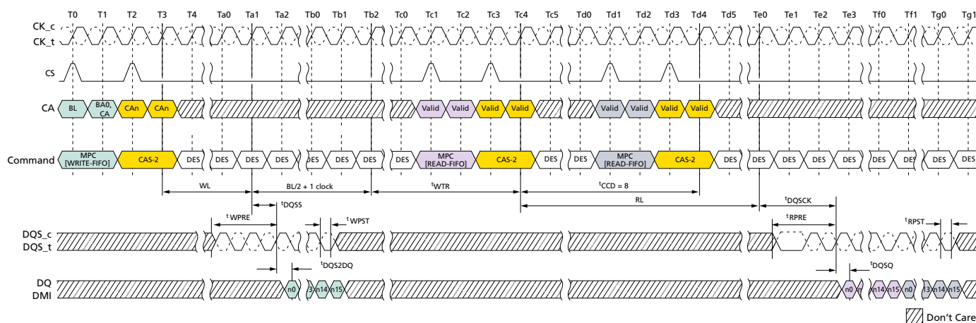
Figure 112: MPC[WRITE-FIFO]-to-MPC[READ-FIFO] Timing
