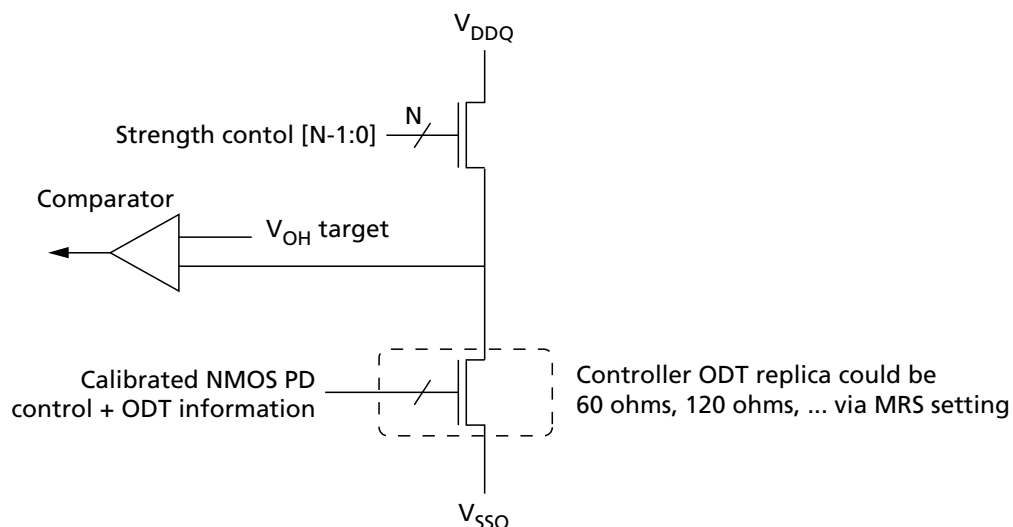
Figure 171: Pull-Up Calibration
