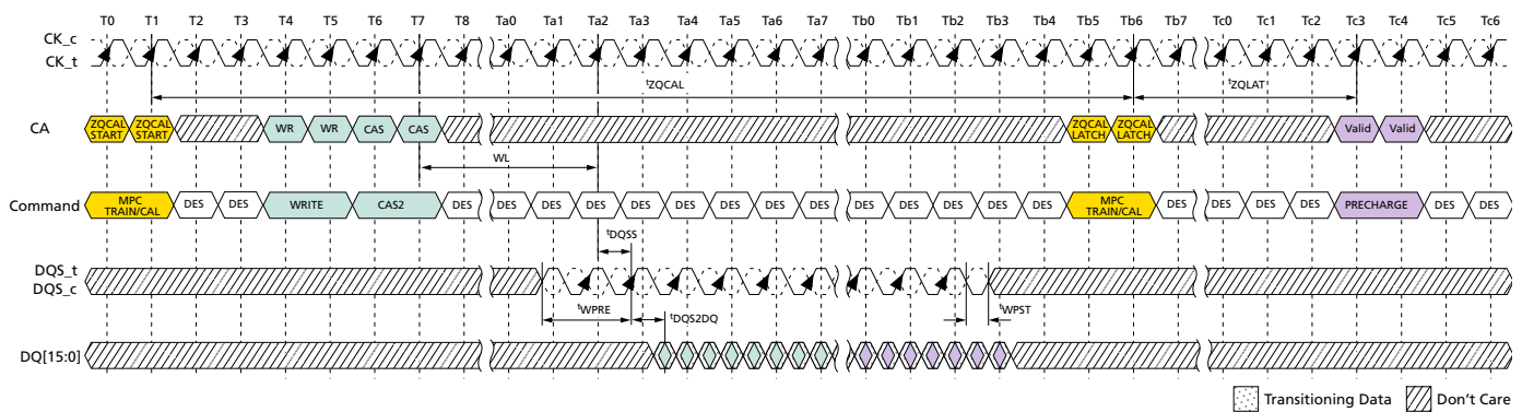
Figure 119: ZQCAL Timing
