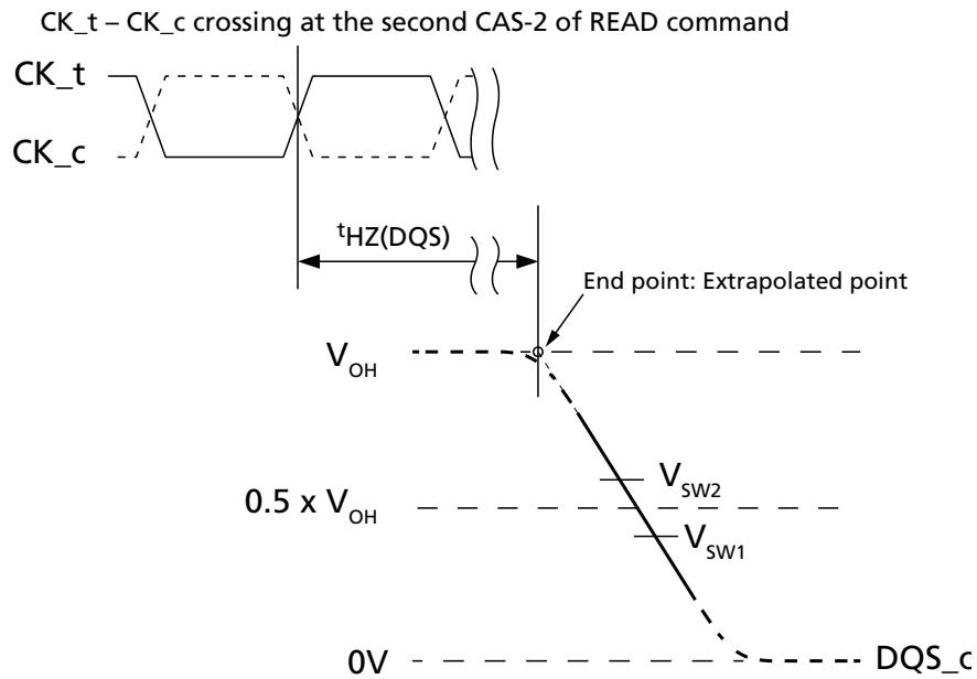
Figure 163: t_{HZ}(DQS) Method for Calculating Transitions and Endpoint
