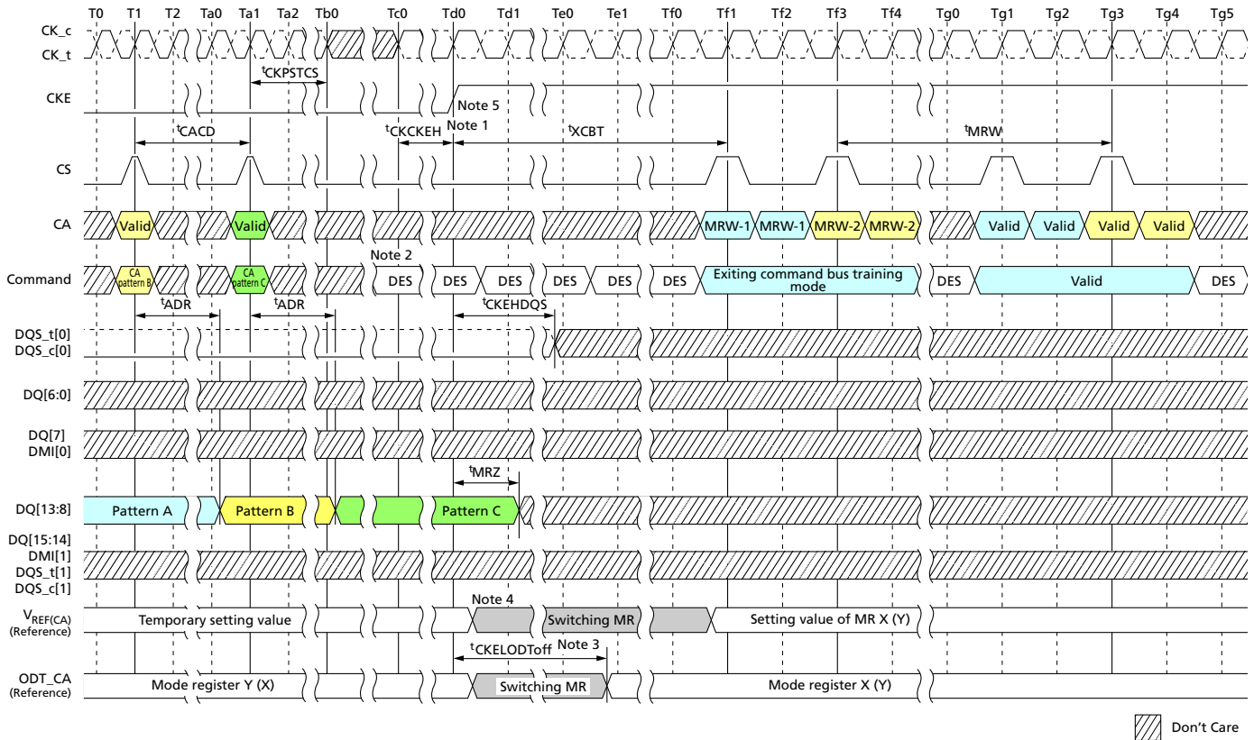
Figure 99: Command Bus Training Mode Exit with Valid Command
