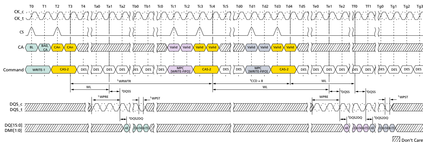
Figure 111: WRITE-to-MPC[WRITE-FIFO] Operation Timing
