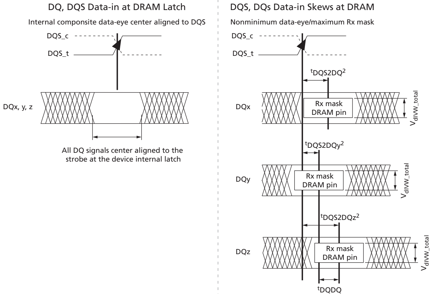
Figure 159: DQ-to-DQS t_{DQS2DQ} and t_{DQDQ}
