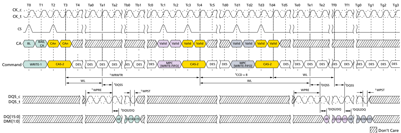
Figure 105: WRITE-FIFO – t_{WPRE} = 2nCK , t_{WPST} = 0.5nCK
