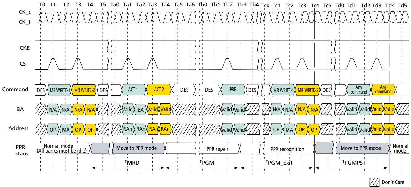
Figure 129: Post-Package Repair Timing
