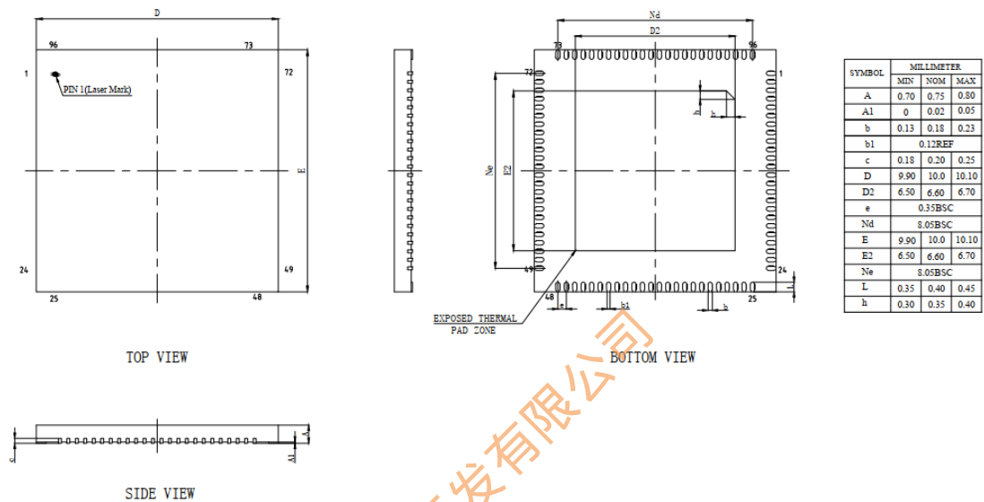
Figure 12. Package Dimensions (QFN96)
