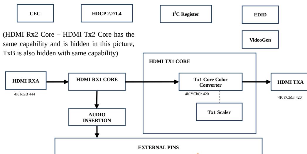
Figure 4. GSV2008 4K 444-to-4K 420 diagram
