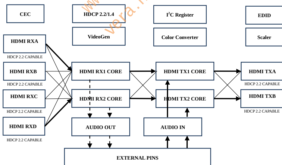
Figure 2. GSV2008 audio insertion diagram
