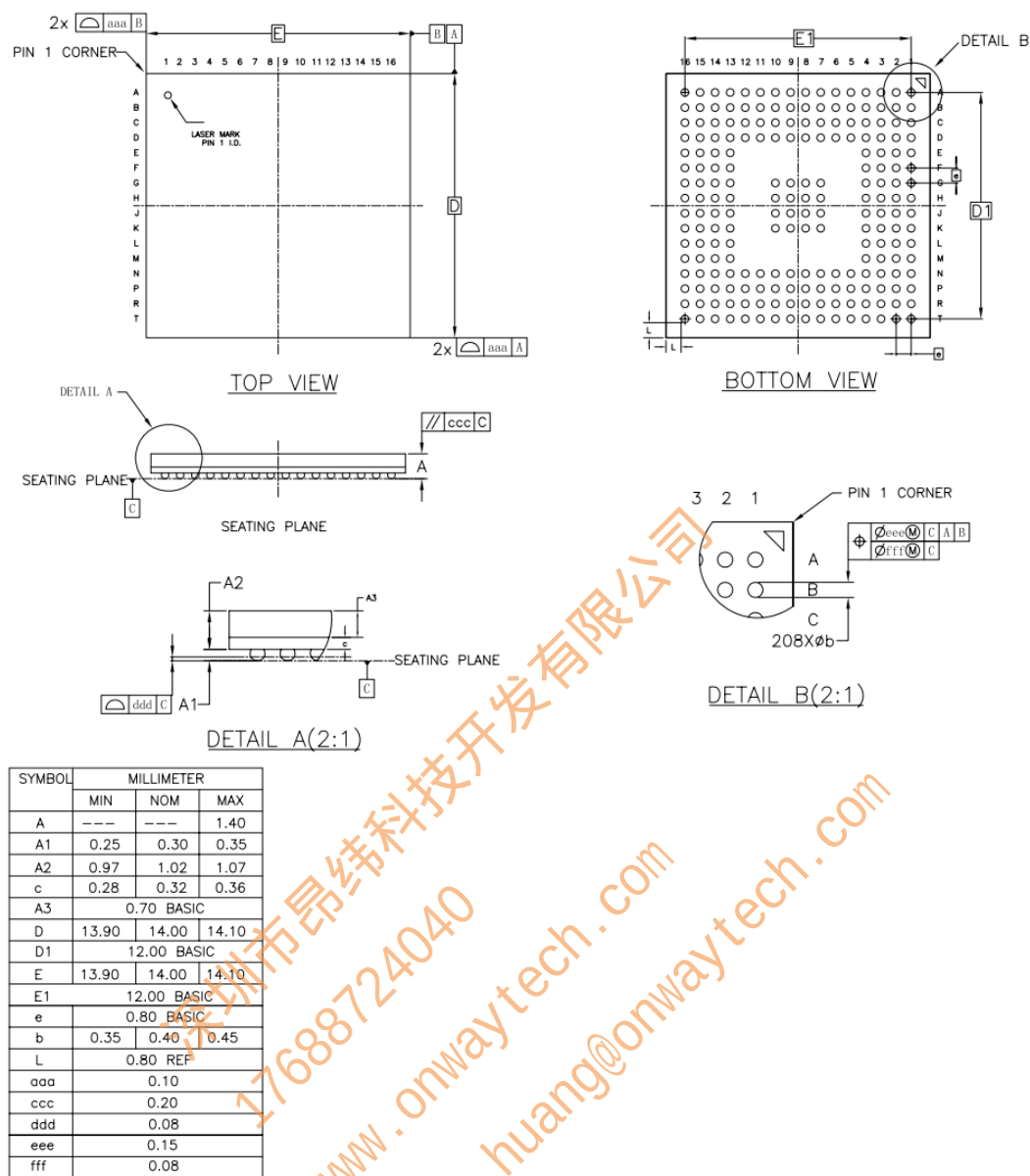
Figure 11. GSV2008 package dimensions
