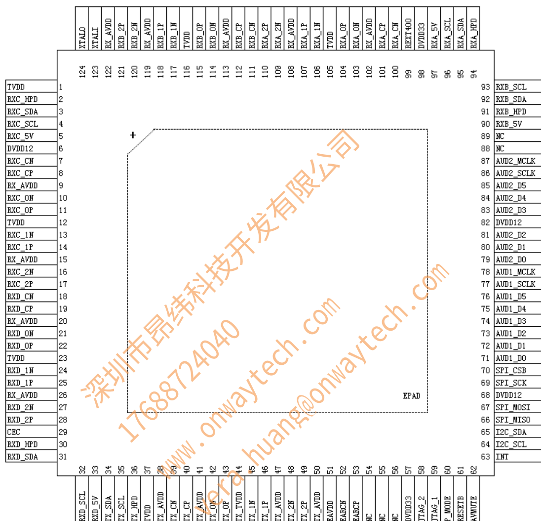
Figure 5. GSV2705 QFN124 Pin Diagram
