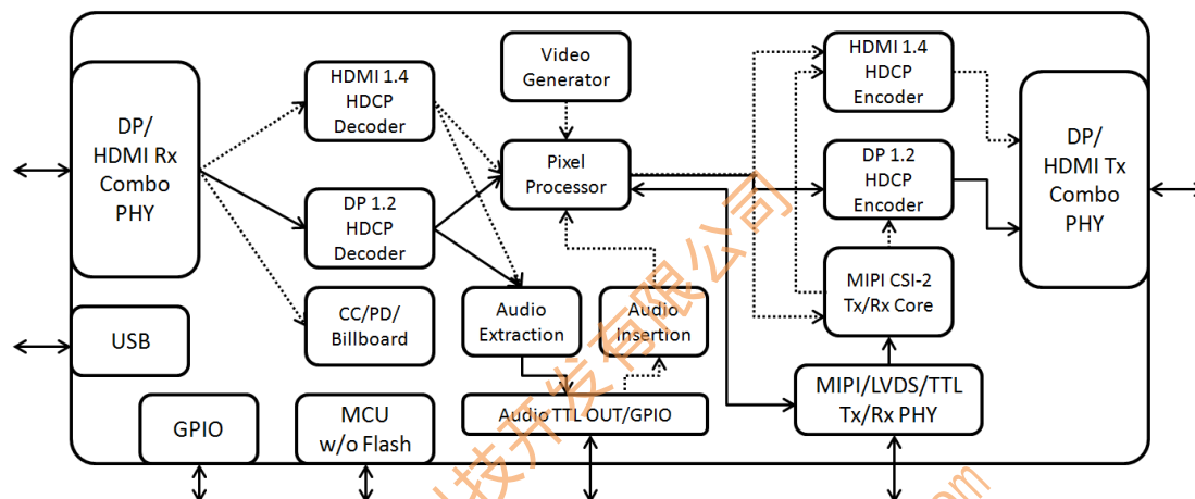
Figure 3. HDMI In to Type-C Alt-Mode Out with MIPI Out Application
