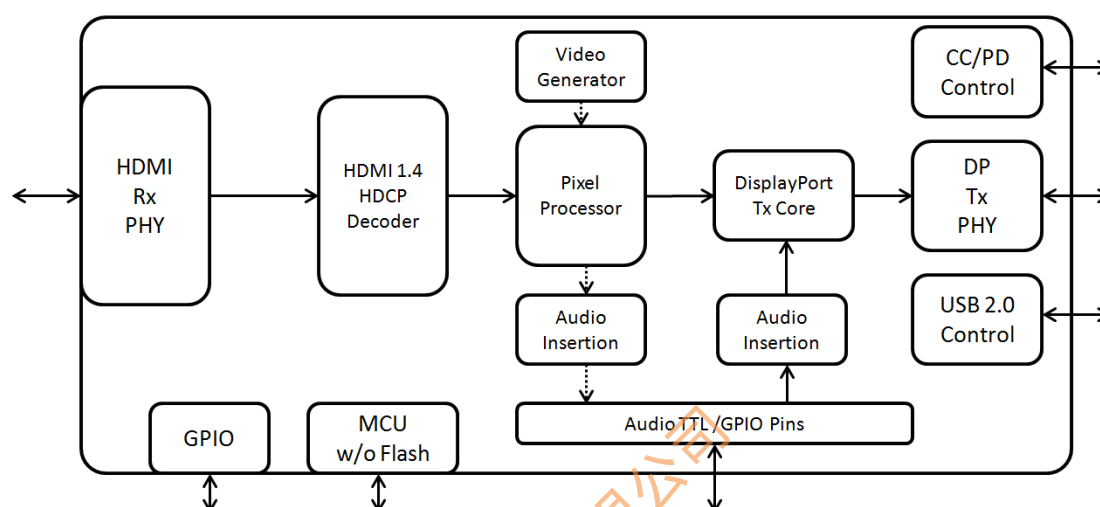
Figure 3. HDMI 1.4 to Type-C Alt-DP Application
