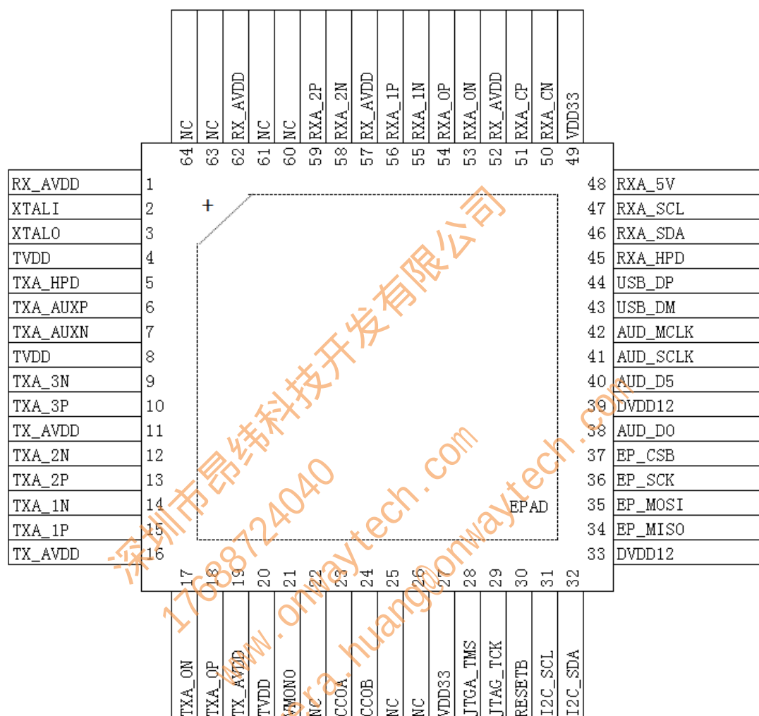
Figure 4. GSV1125 QFN64 Pin Diagram
