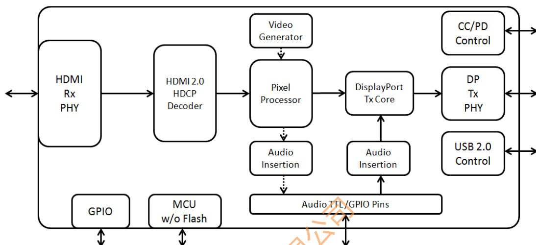
Figure 3. HDMI 2.0 to Type-C Alt-DP Application
