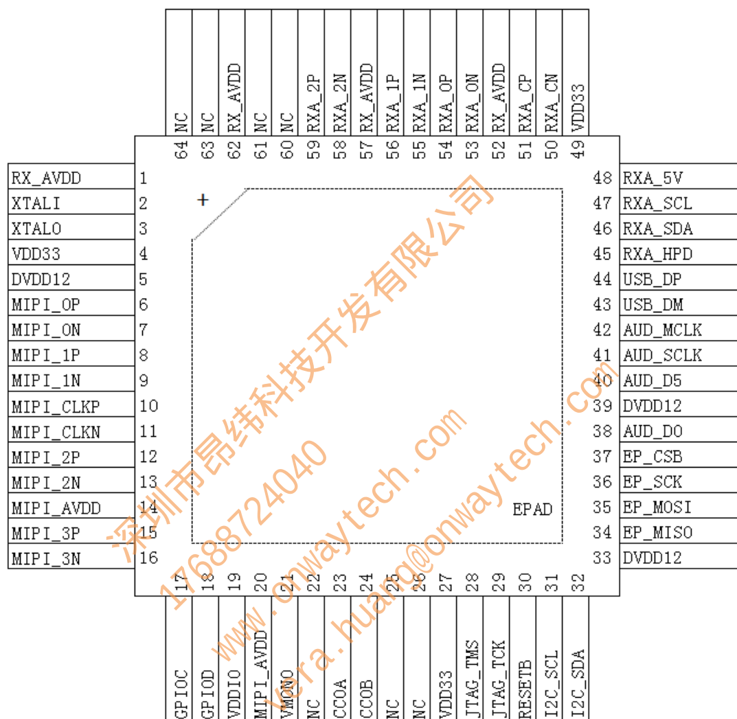
Figure 4. GSV6127 QFN64 Pin Diagram
