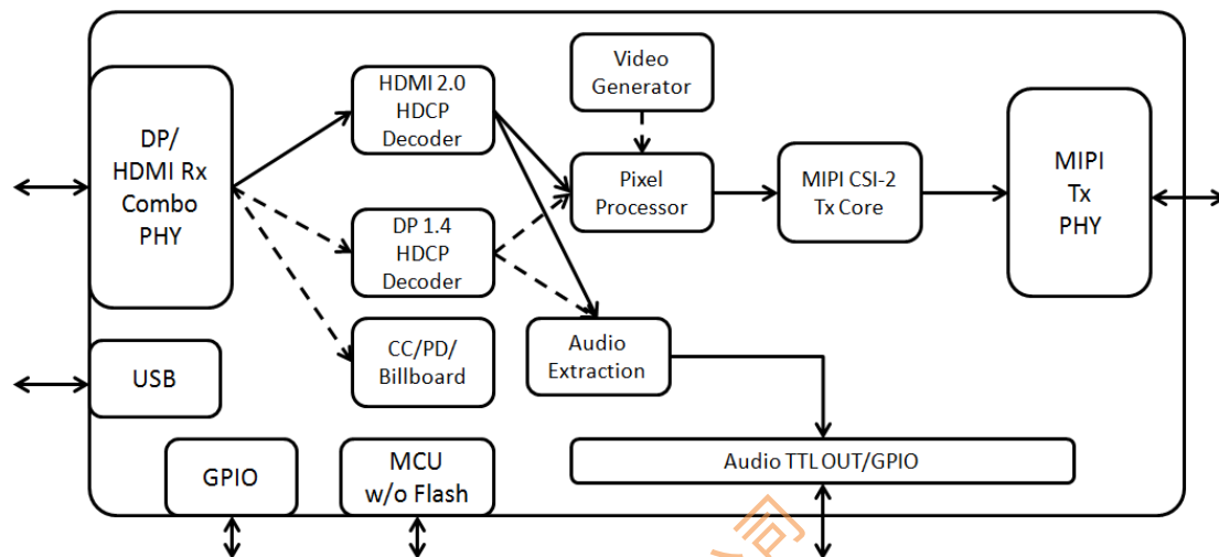
Figure 3. HDMI 2.0 to MIPI CSI-2 Application
