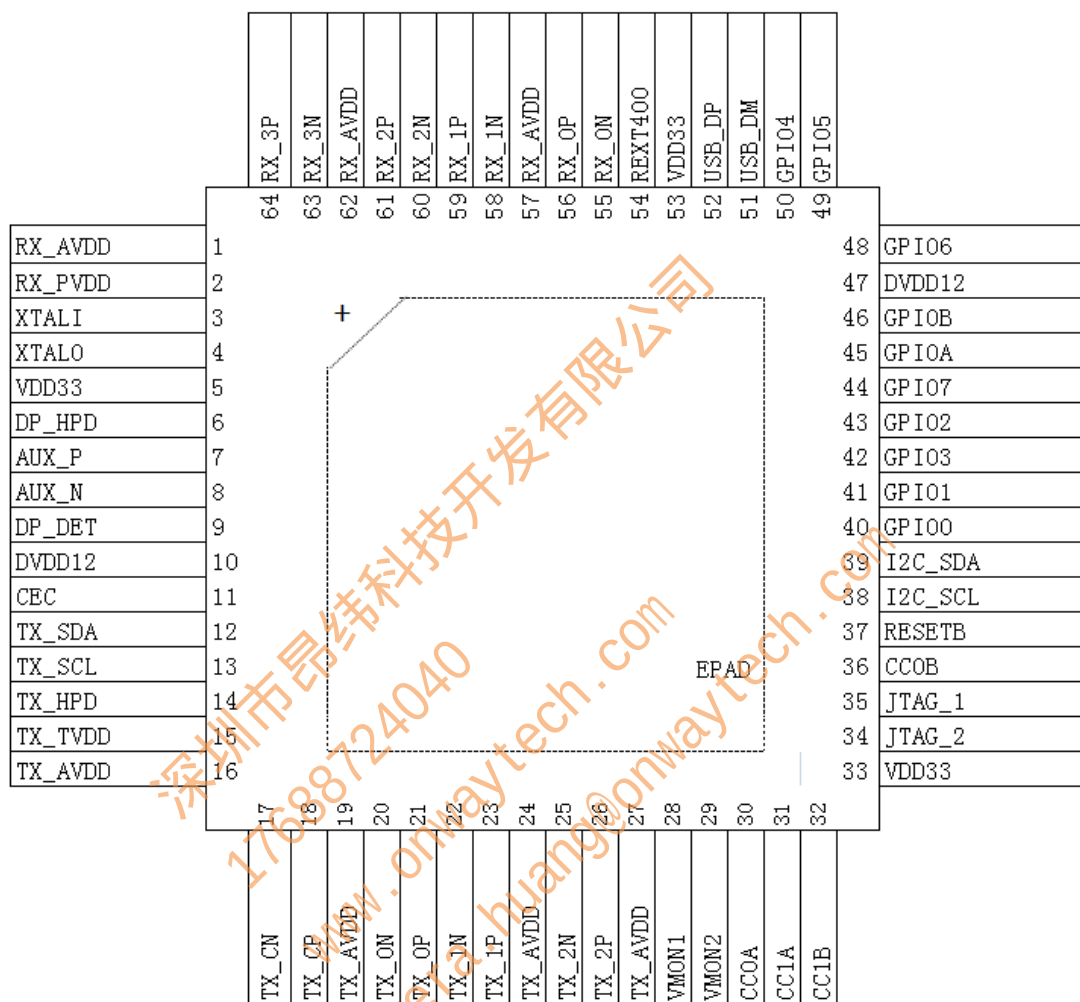
Figure 3. GSV1202E QFN64 Pin Diagram
